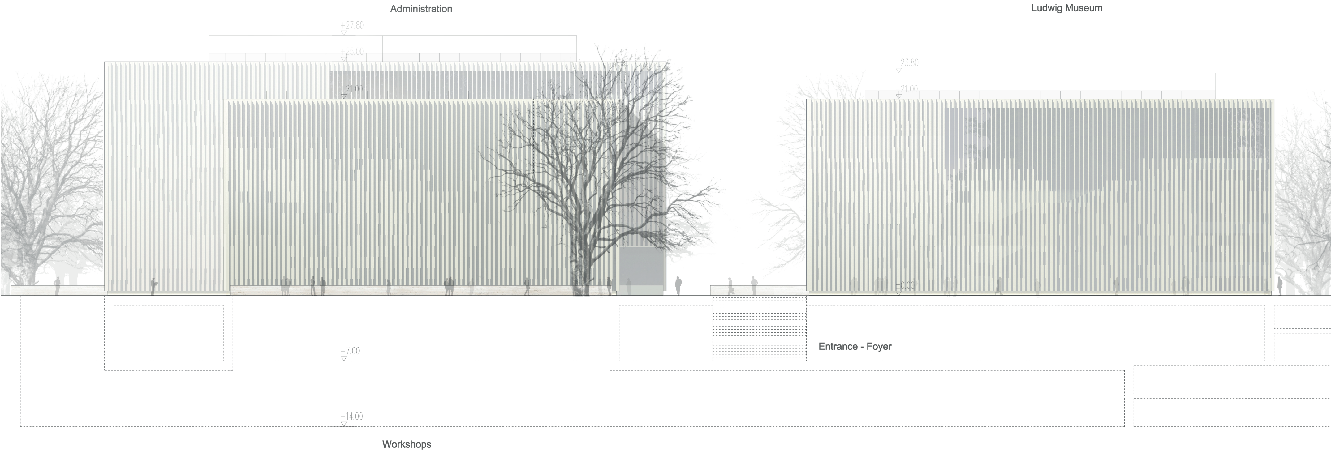
Southwest elevation1:250
