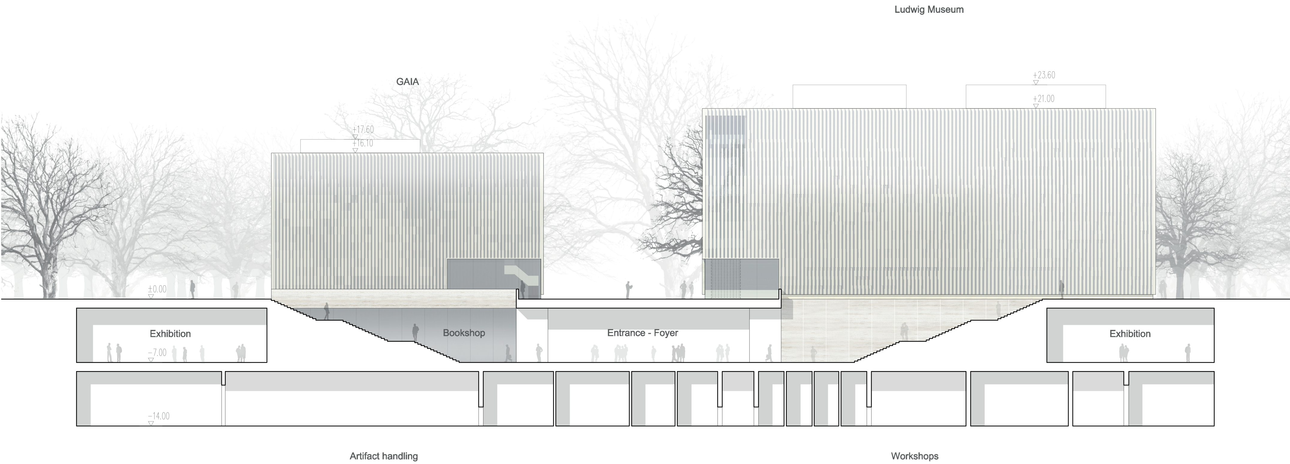
Section AA 1:250
