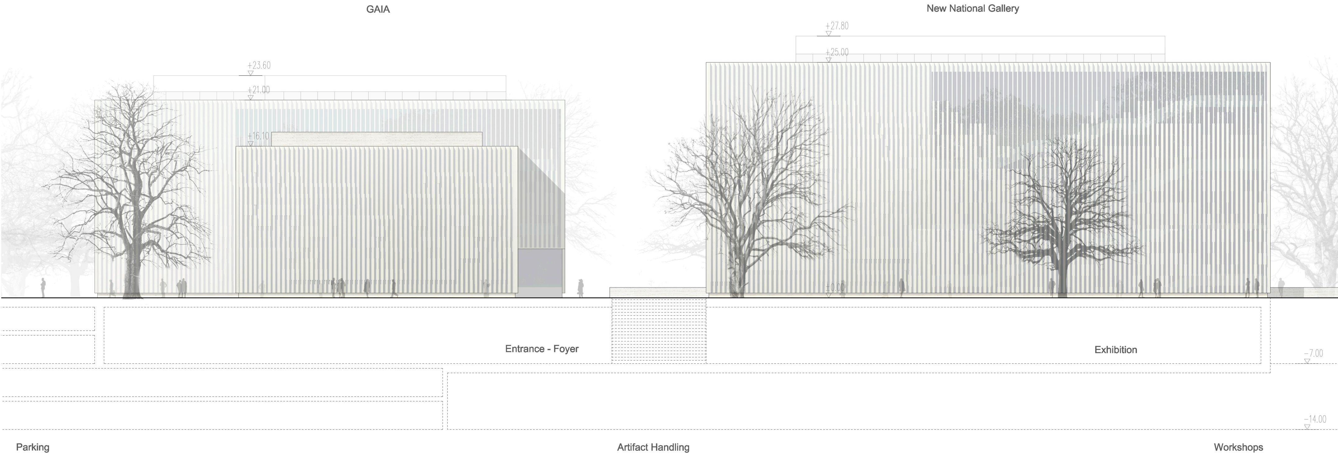
Northeast elevation1:250
